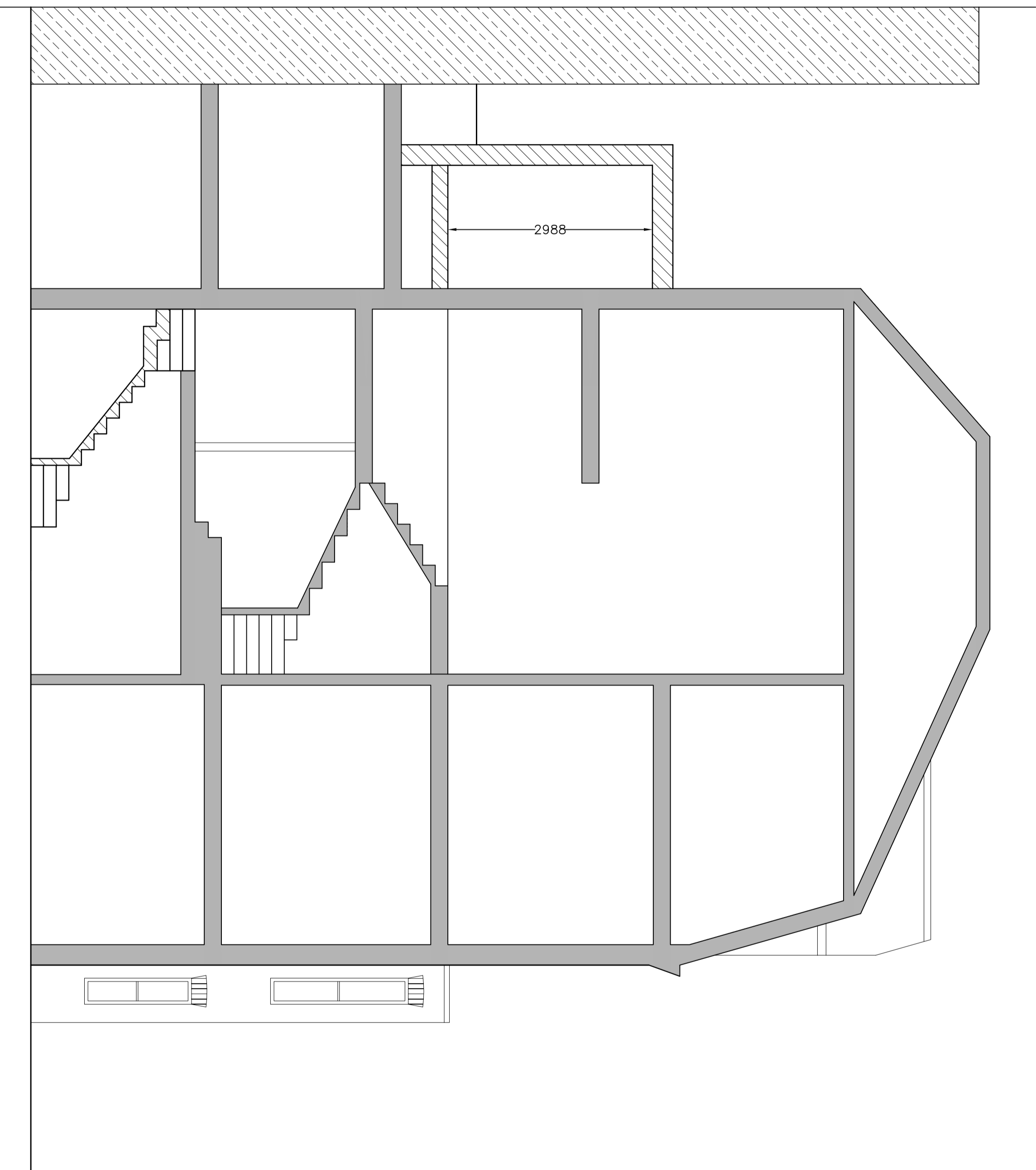
Section A-A Proposed
