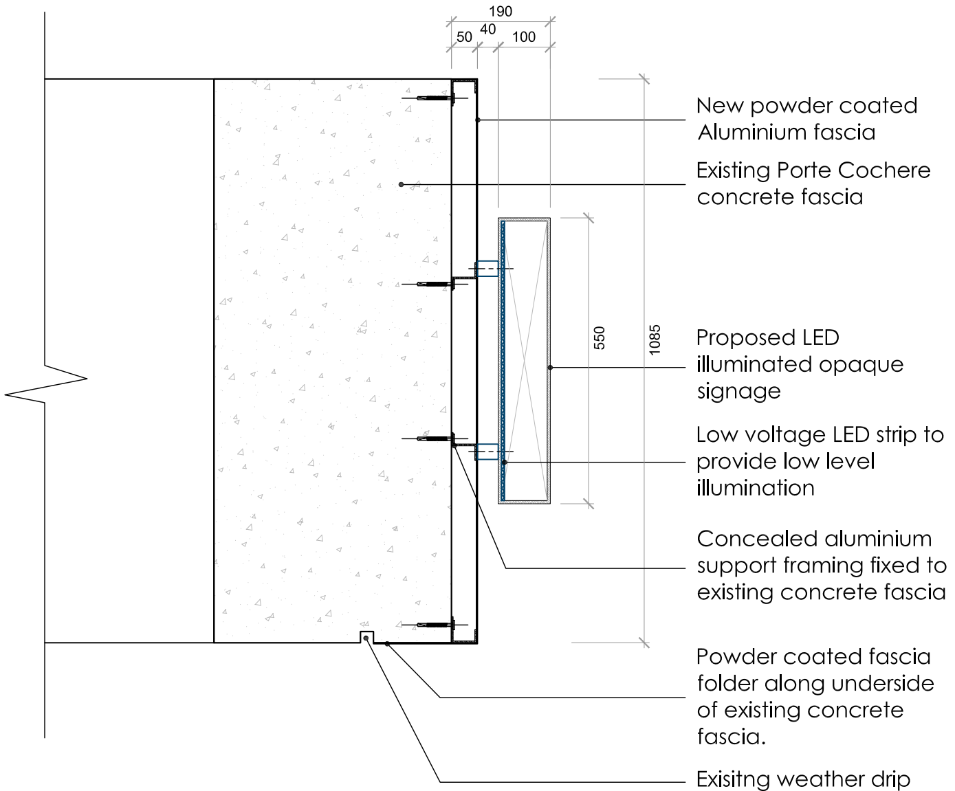
1 SIGNAGE - DETAIL SECTION Scale: 1:10 @ A4
