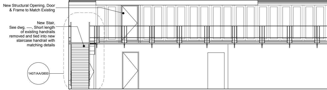
ELEVATION 2: FIRST FLOOR WING A
