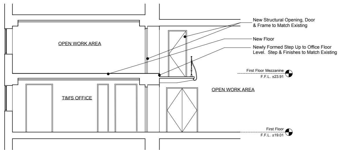
SECTION D-D FIRST FLOOR
