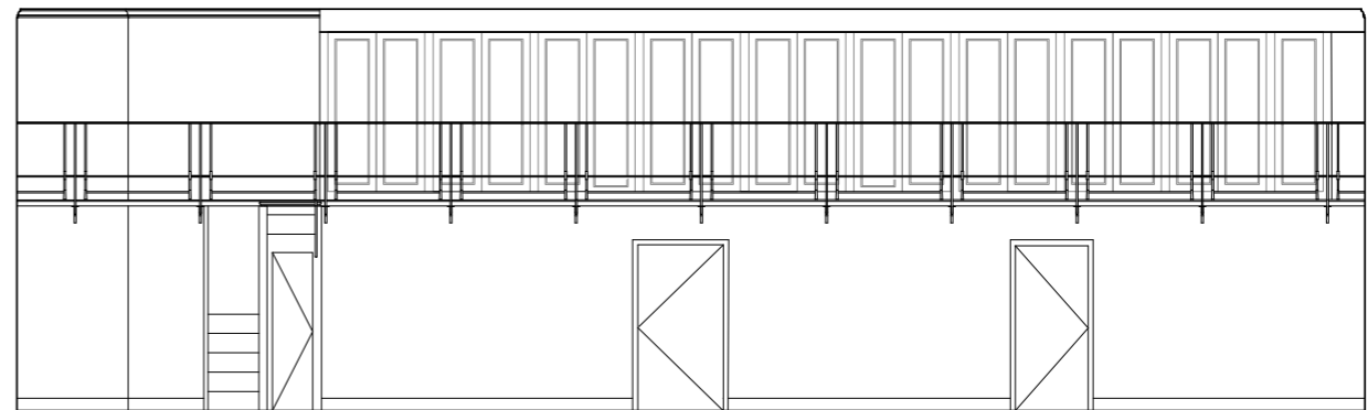
ELEVATION 3: FIRST FLOOR WING A
