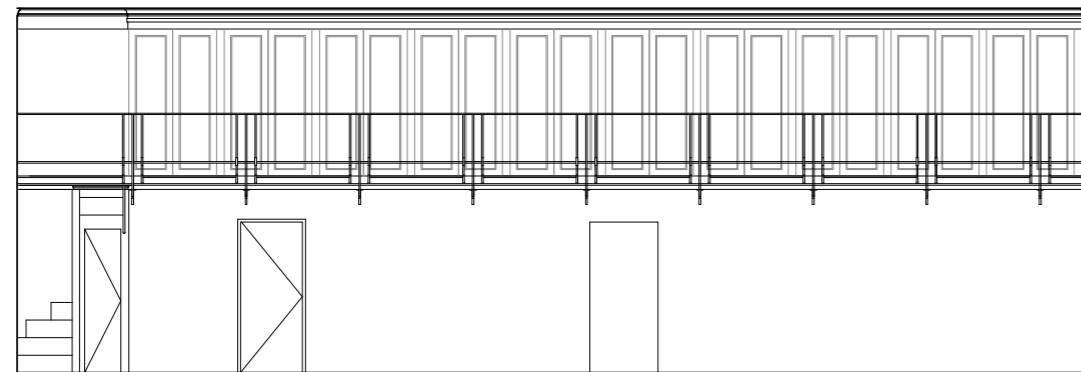
ELEVATION 2: FIRST FLOOR WING A
