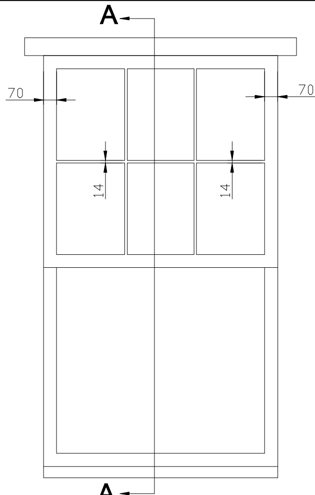
Example Existing Timber Sash
