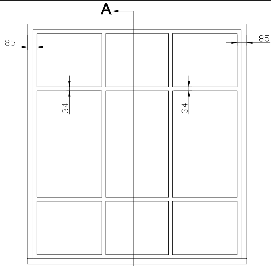
Example Existing Metal Casement
