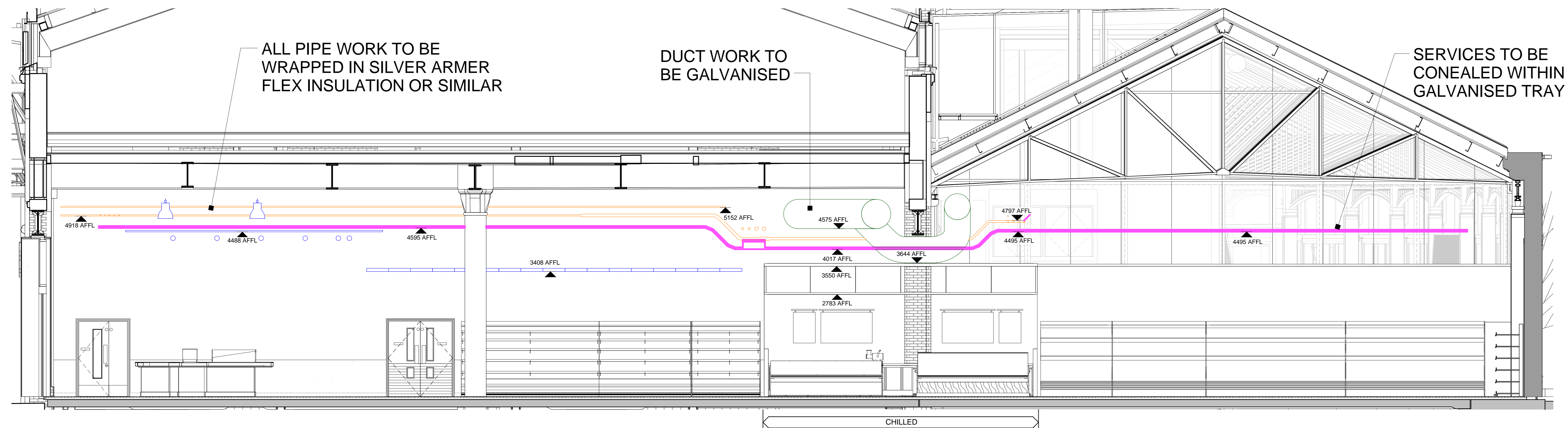
1 INTERNAL ELEVATION OF WAITROSE SALES FLOOR 01 1 : 50
