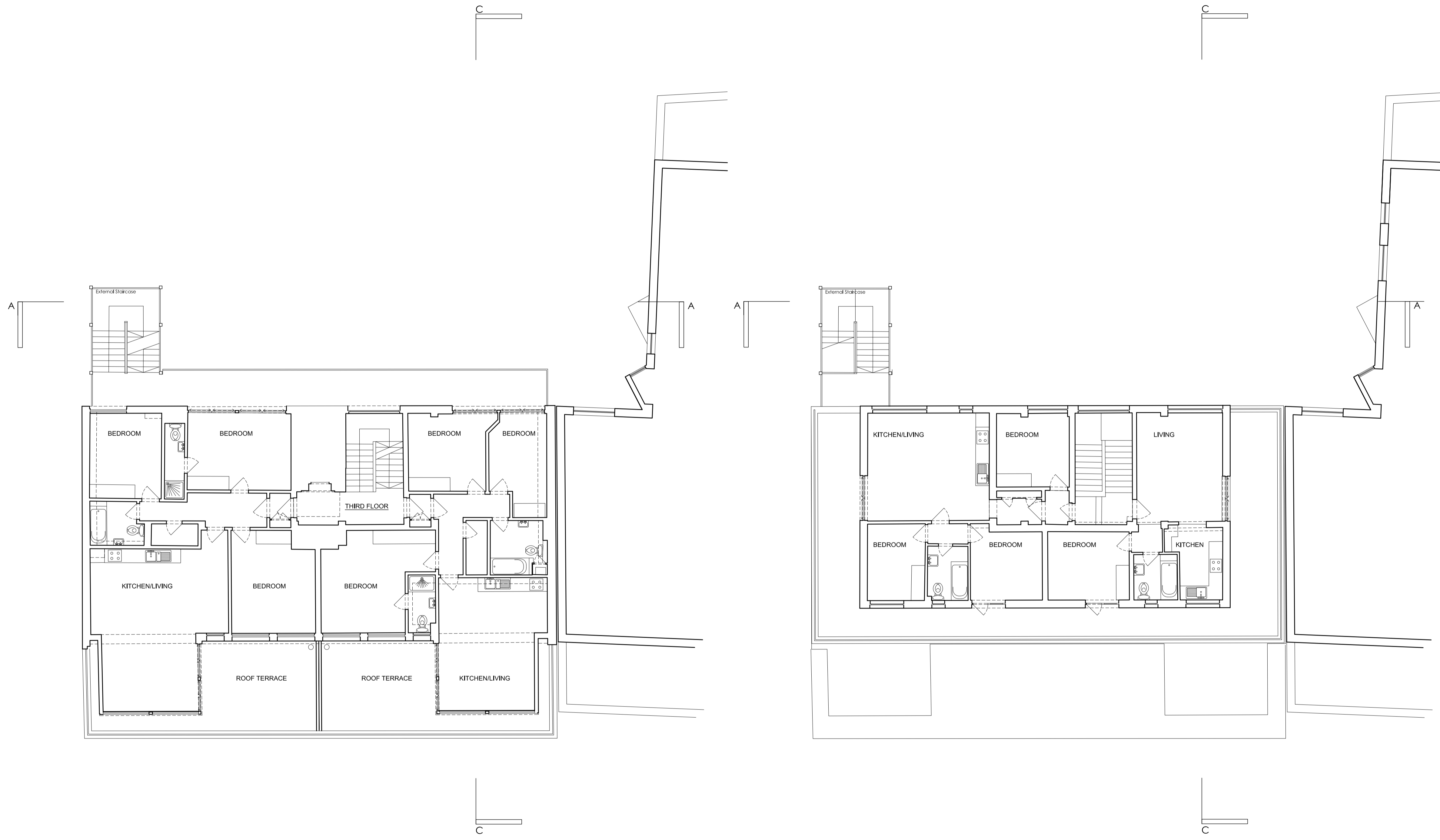
THIRD FLOOR
