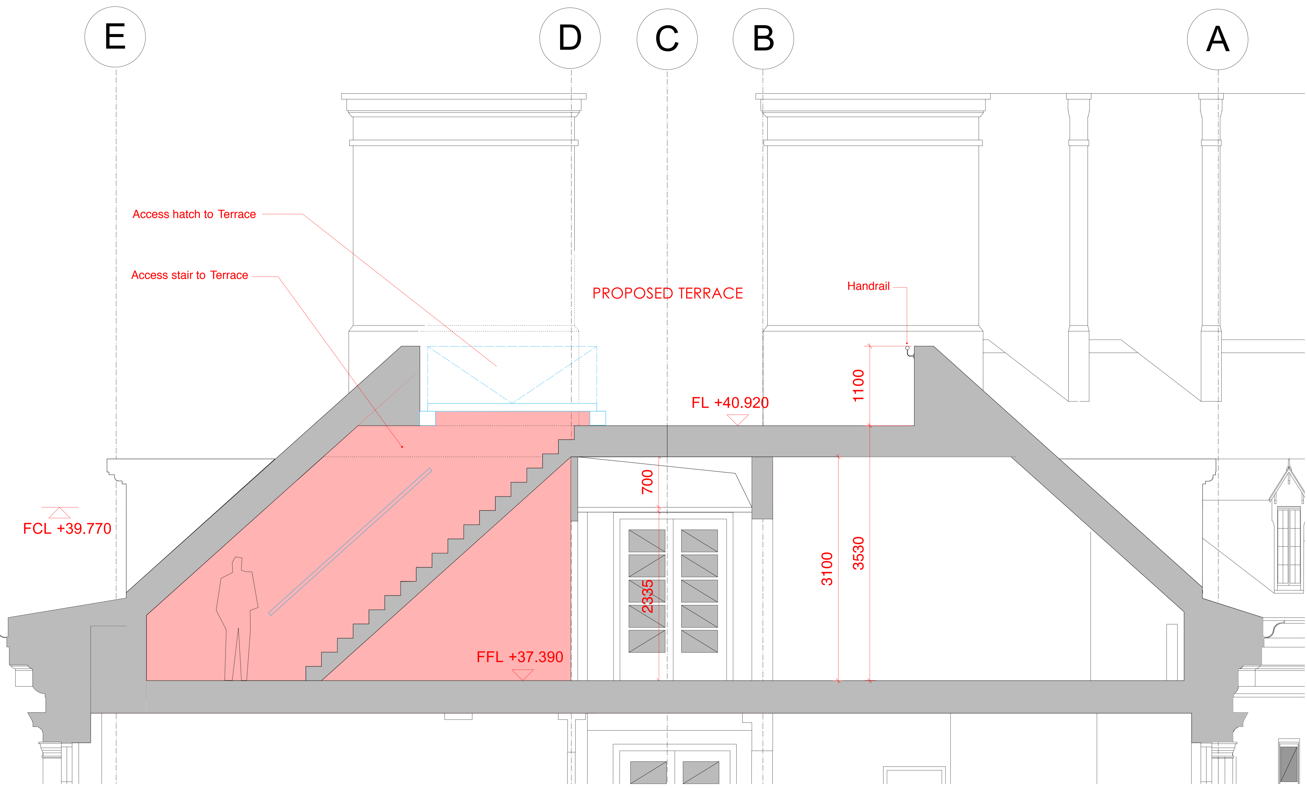
X-SECTION
