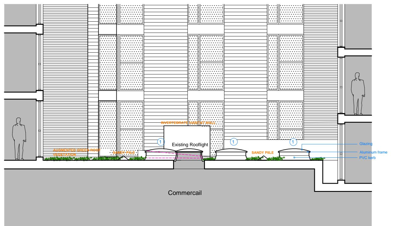
LONG SECTION YY - PROPOSED
