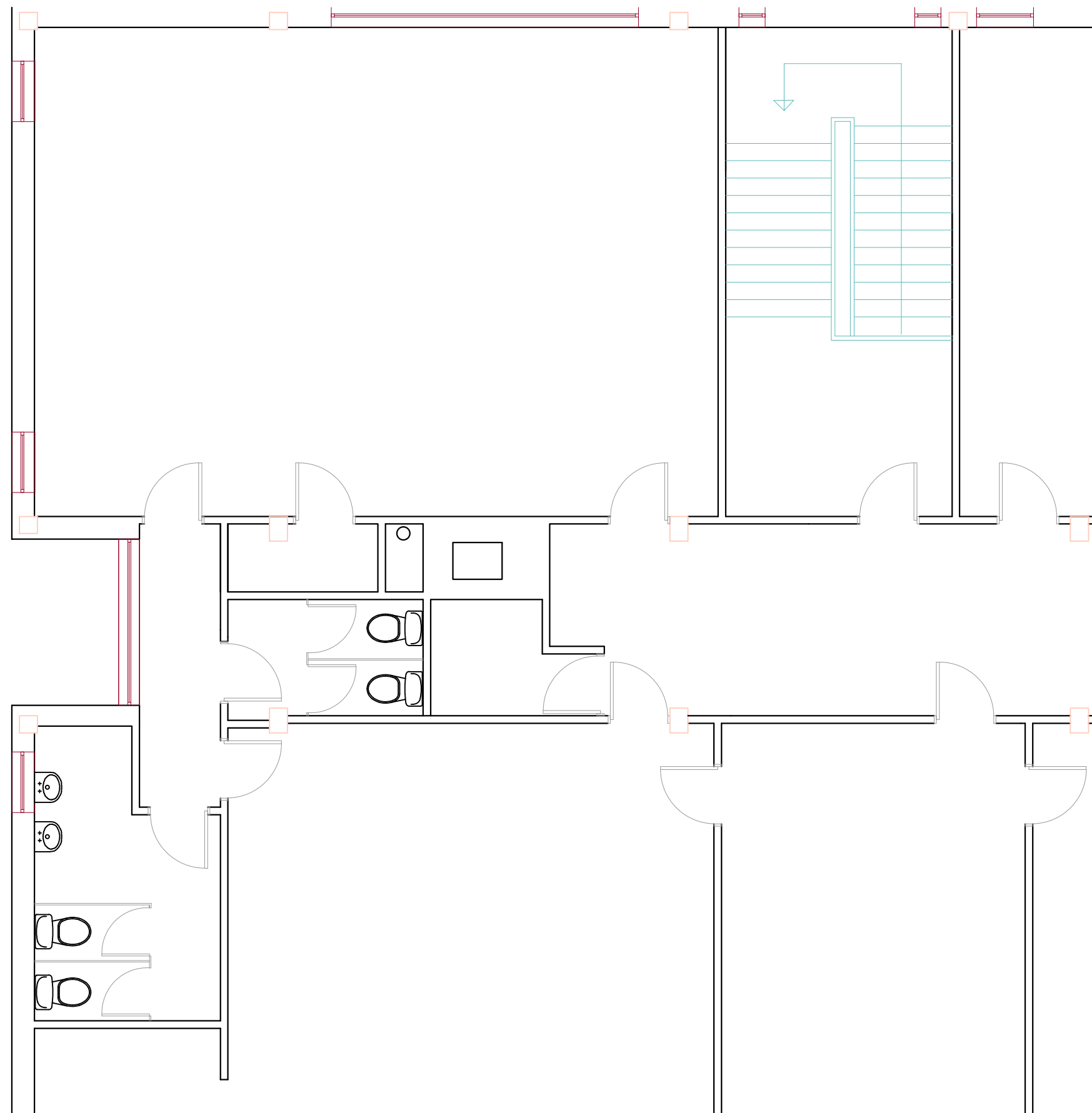
SECOND FLOOR PLAN AS EXISTING
