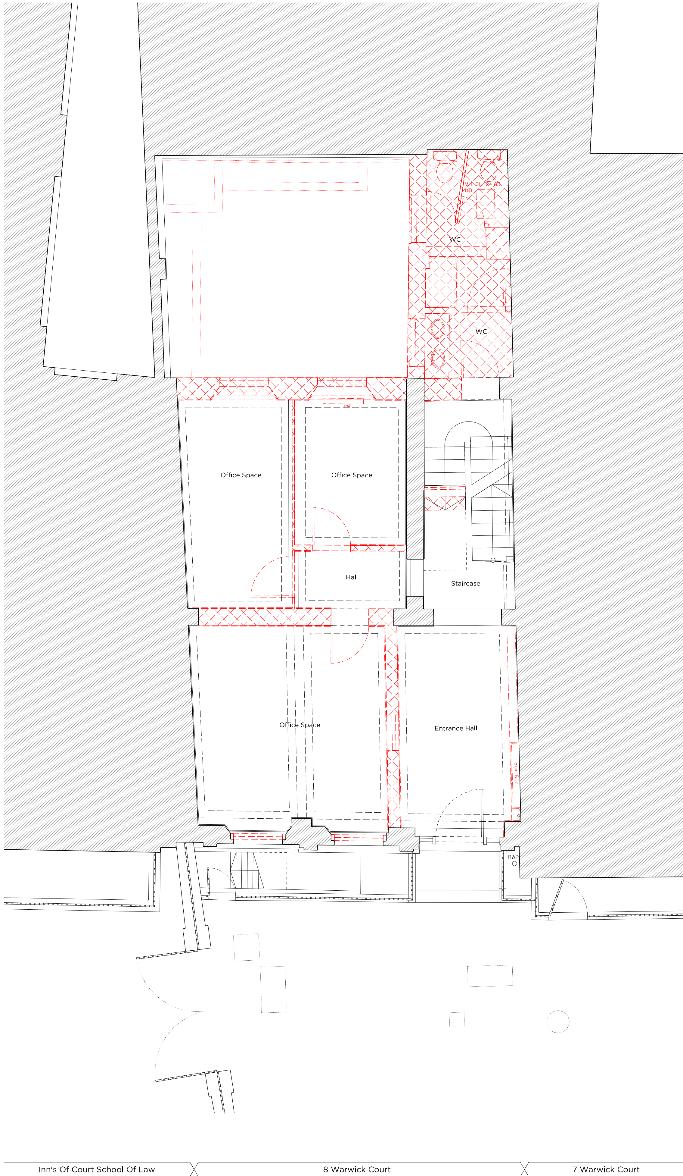
DEMOLITION GROUND FLOOR
