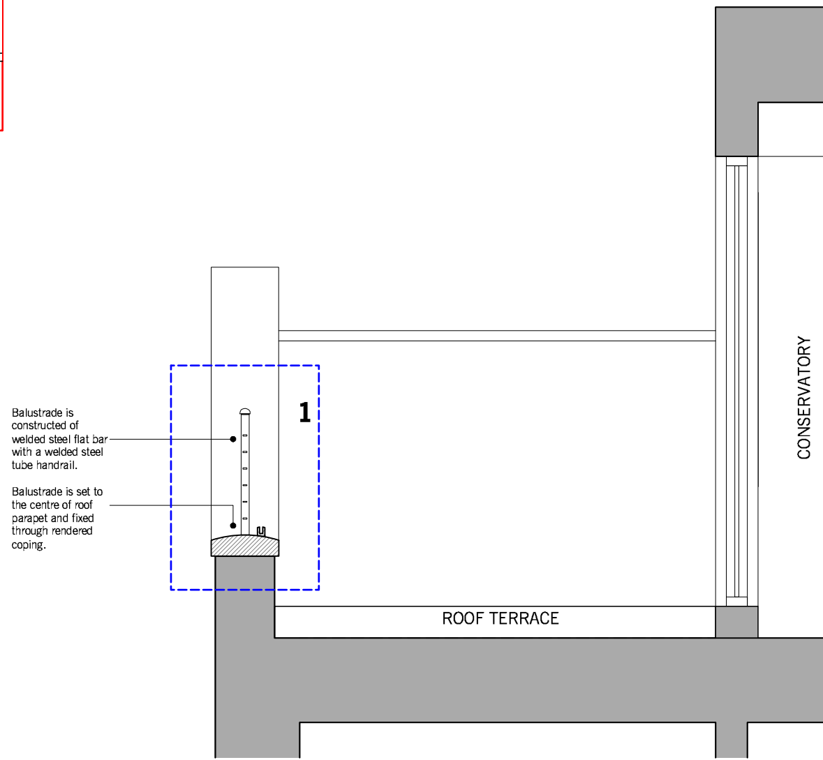
EXISTING - Scale 1:25
