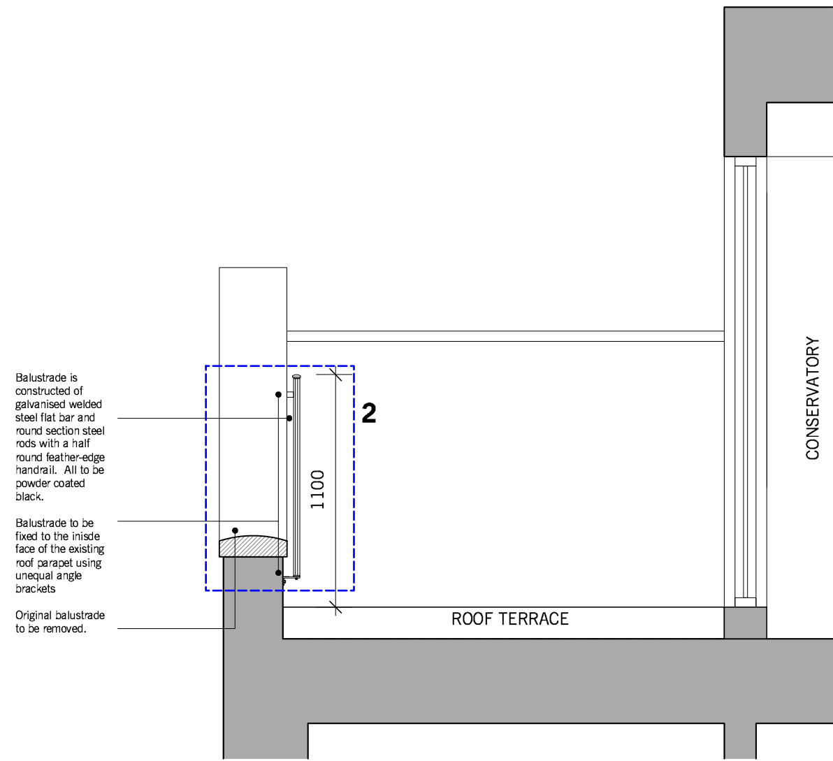
PROPOSED - Scale 1:25
