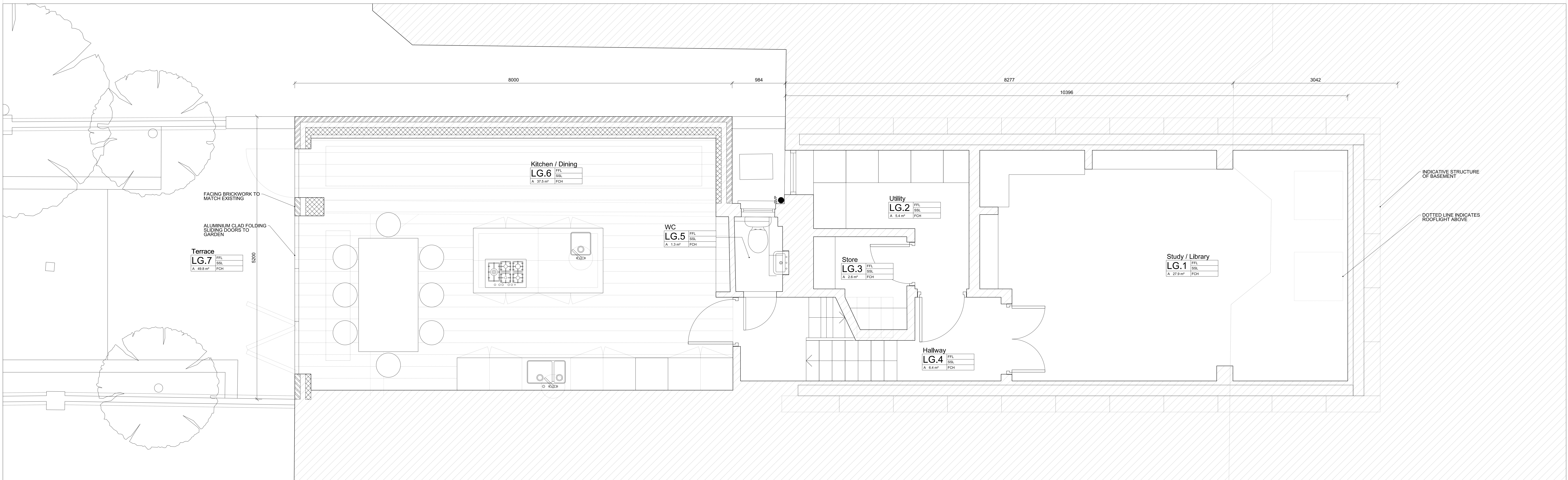
1 PLAN 1:25/50/100 @ A0/A2/A4 Basement - Proposed
