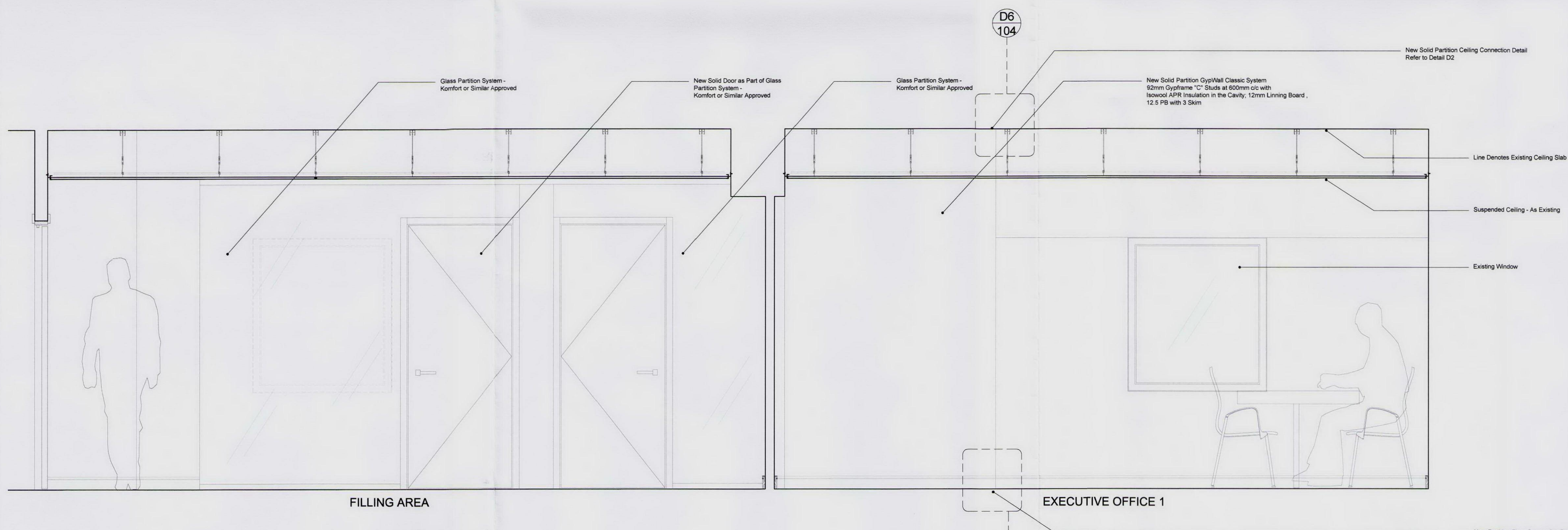
PROPOSED SECTION CC - FIRST FLOOR FILLING AREA/ EXECUTIVE OFFICES SCALE 1:20 @ A1
