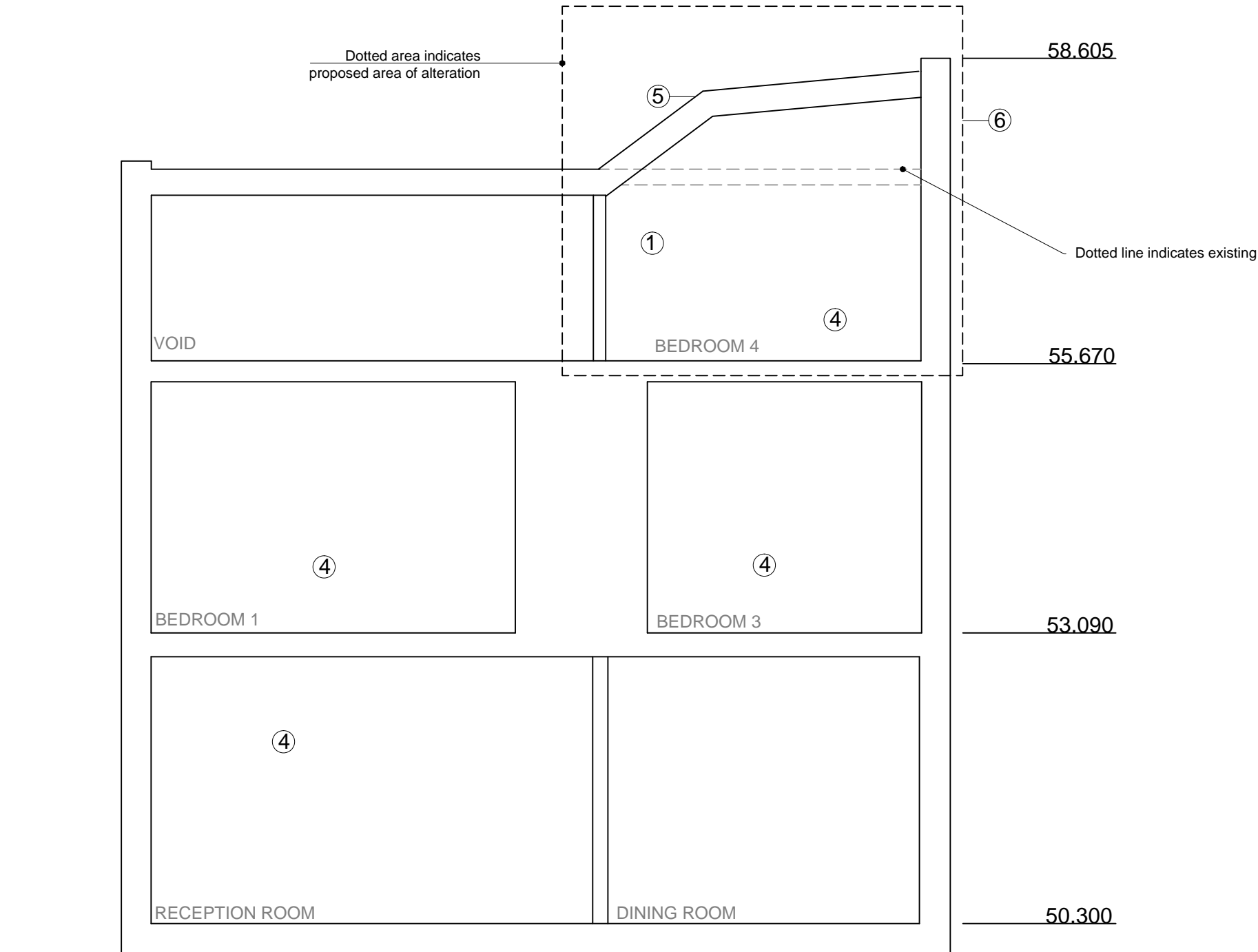
SECTION C PROPOSED
