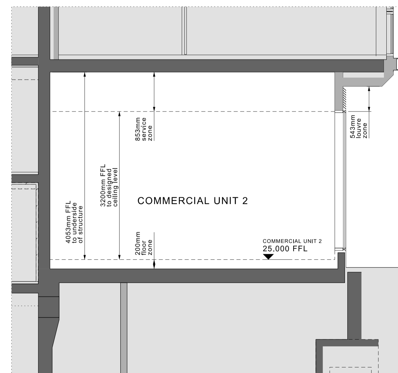
SECTION C-C
