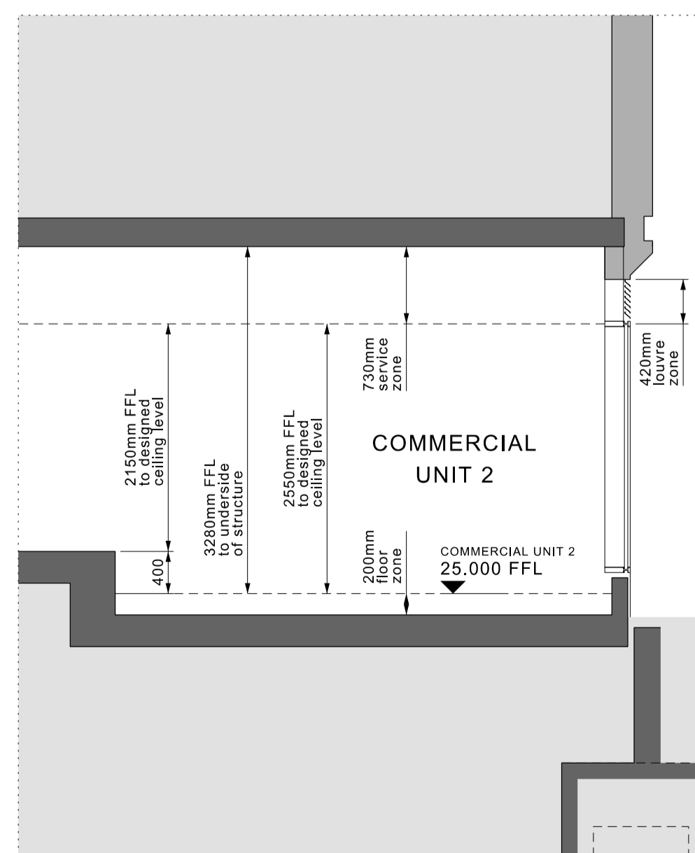
SECTION B-B
