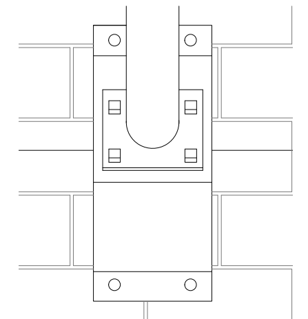
6 Elevation detail of existing flag pole 2001
