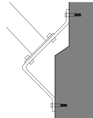
5 Section detail of existing flag pole 2001
