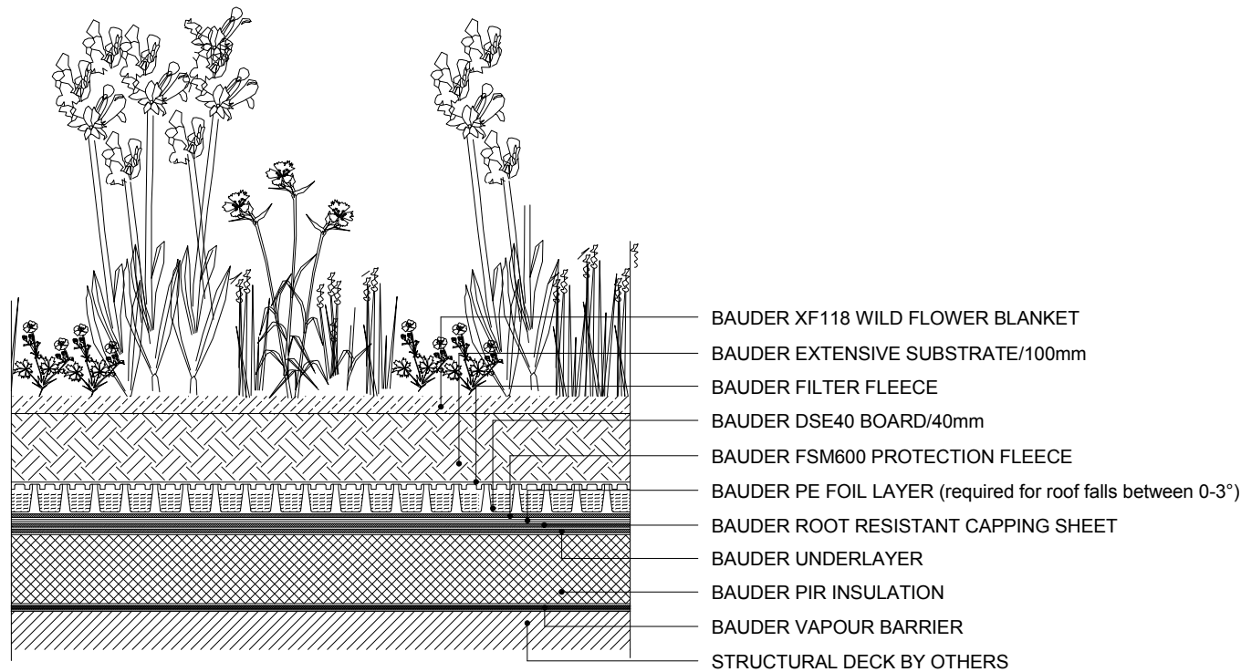
2 GREEN ROOF DETAIL SECTION 1:10
