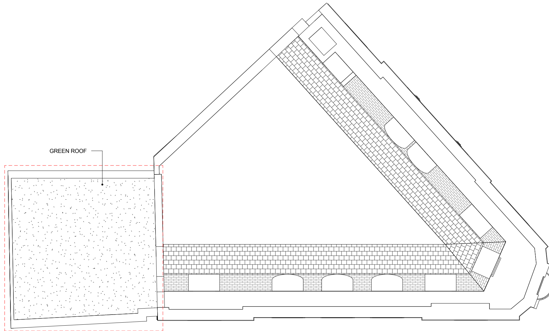
1 ROOF PLAN 1:100
