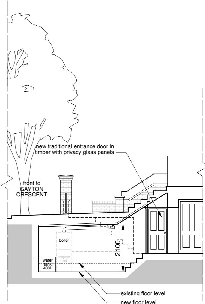
SECTION B PROPOSED
