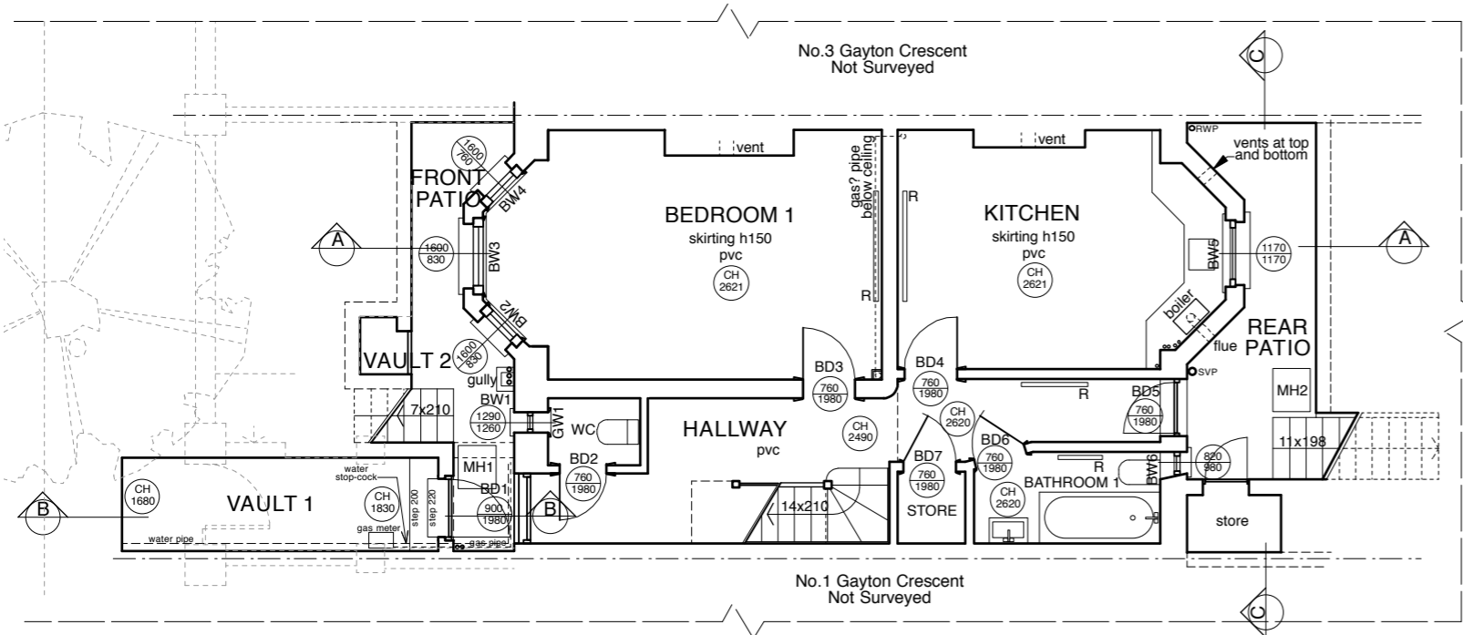
LOWER GROUND FLOOR PLAN - EXISTING
