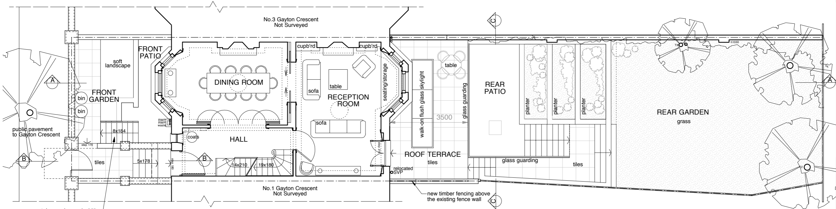
GROUND FLOOR PLAN - PROPOSED
