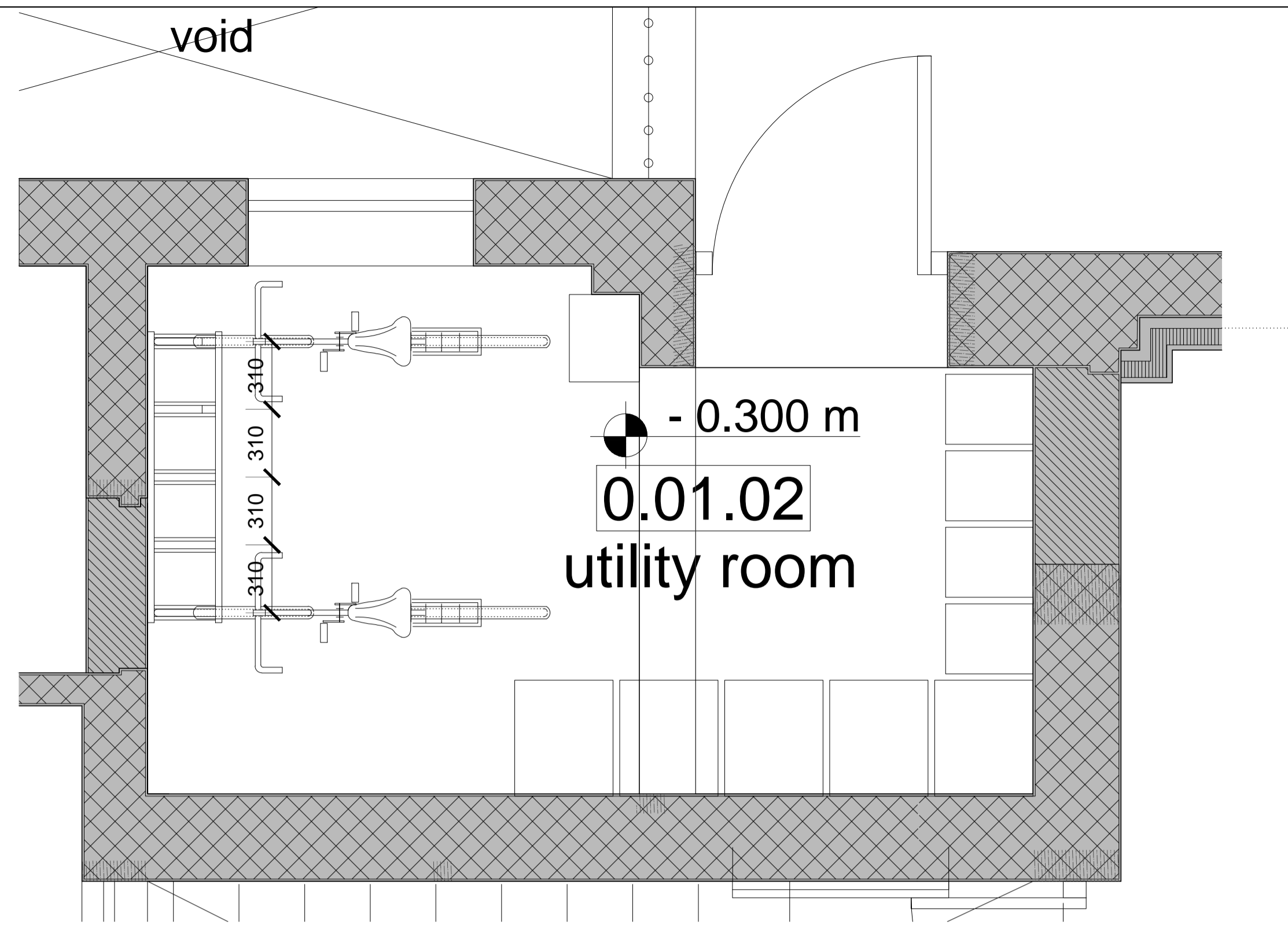
2 BIKE STORE - PLAN - FLOOR STANDS 1/20
