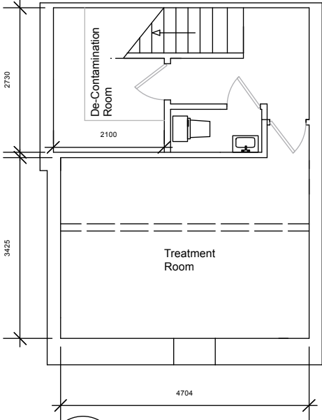
Proposed Basement Scale: 1:100
