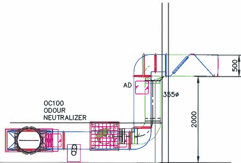
SECTION ON ARROW A
