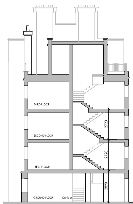
EXISTING STAIR SECTION
