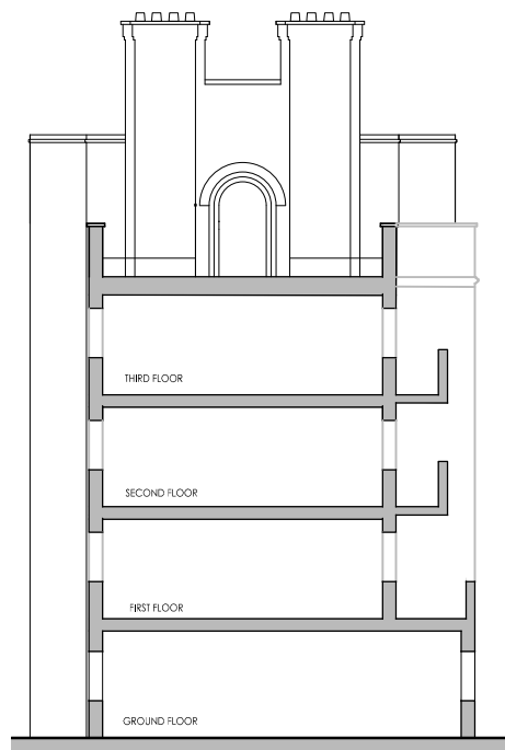
EXISTING CROSS SECTION
