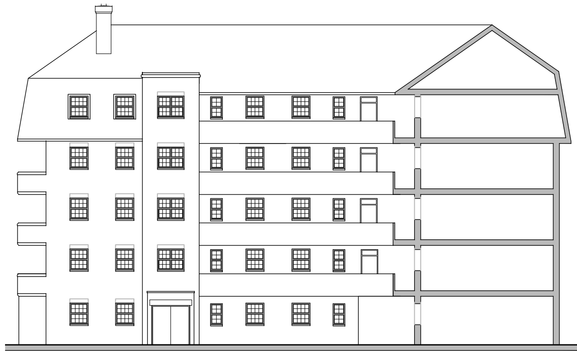
EXISTING ELEVATION TO ALDENHAM STREET
