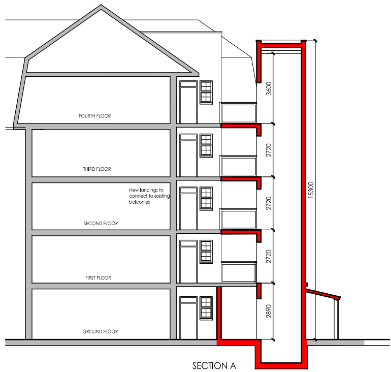
SECTION A
