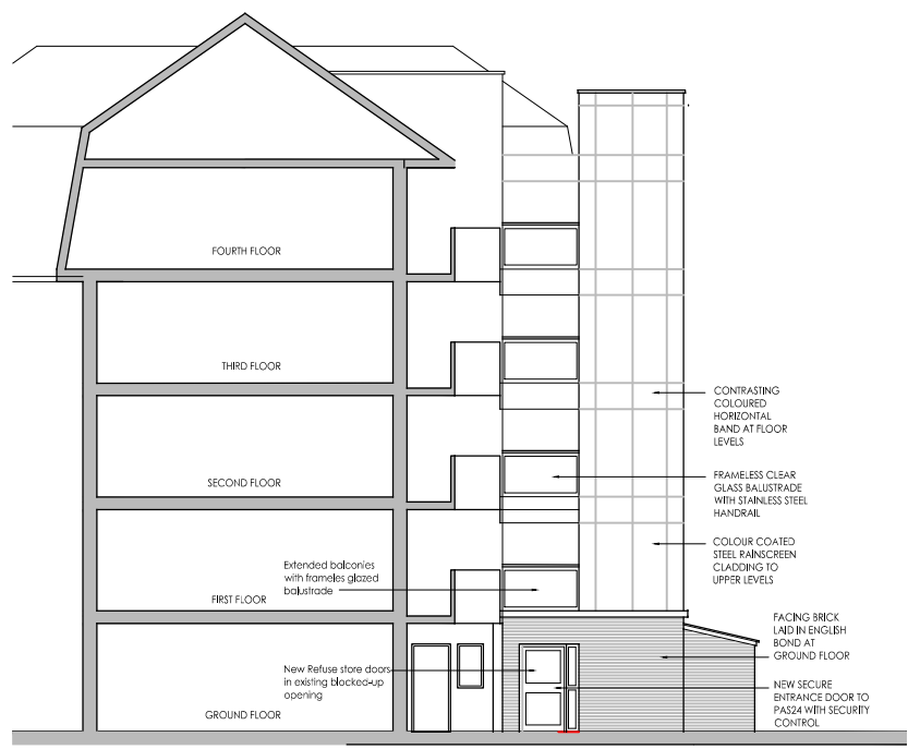
NEW SOUTH SIDE ELEVATION
