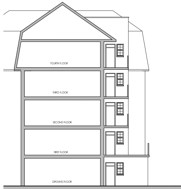
EXISTING CROSS SECTION
