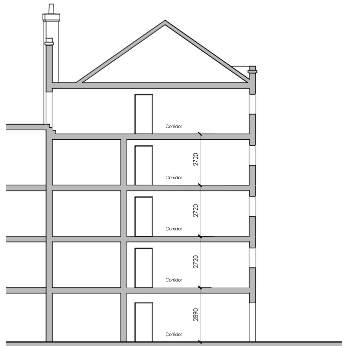
SECTION A
