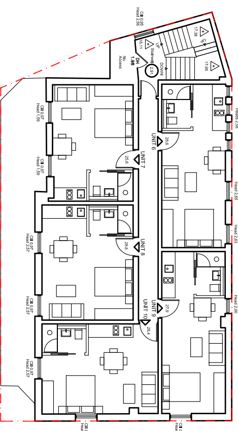
SECOND LEVEL PLAN 1:200 SCALE
