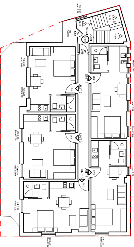
FIRST LEVEL PLAN 1:200 SCALE
