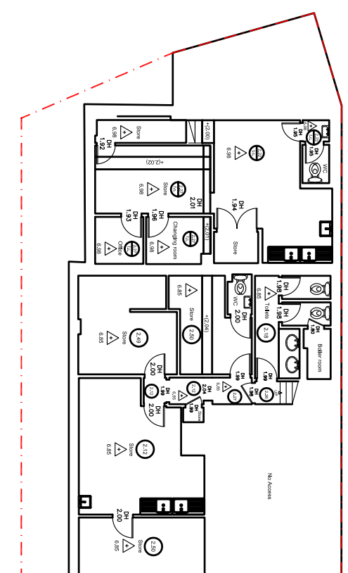
BASEMENT LEVEL PLAN 1:200 SCALE
