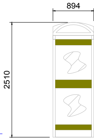
FRONT ELEVATION Scale 1:50
