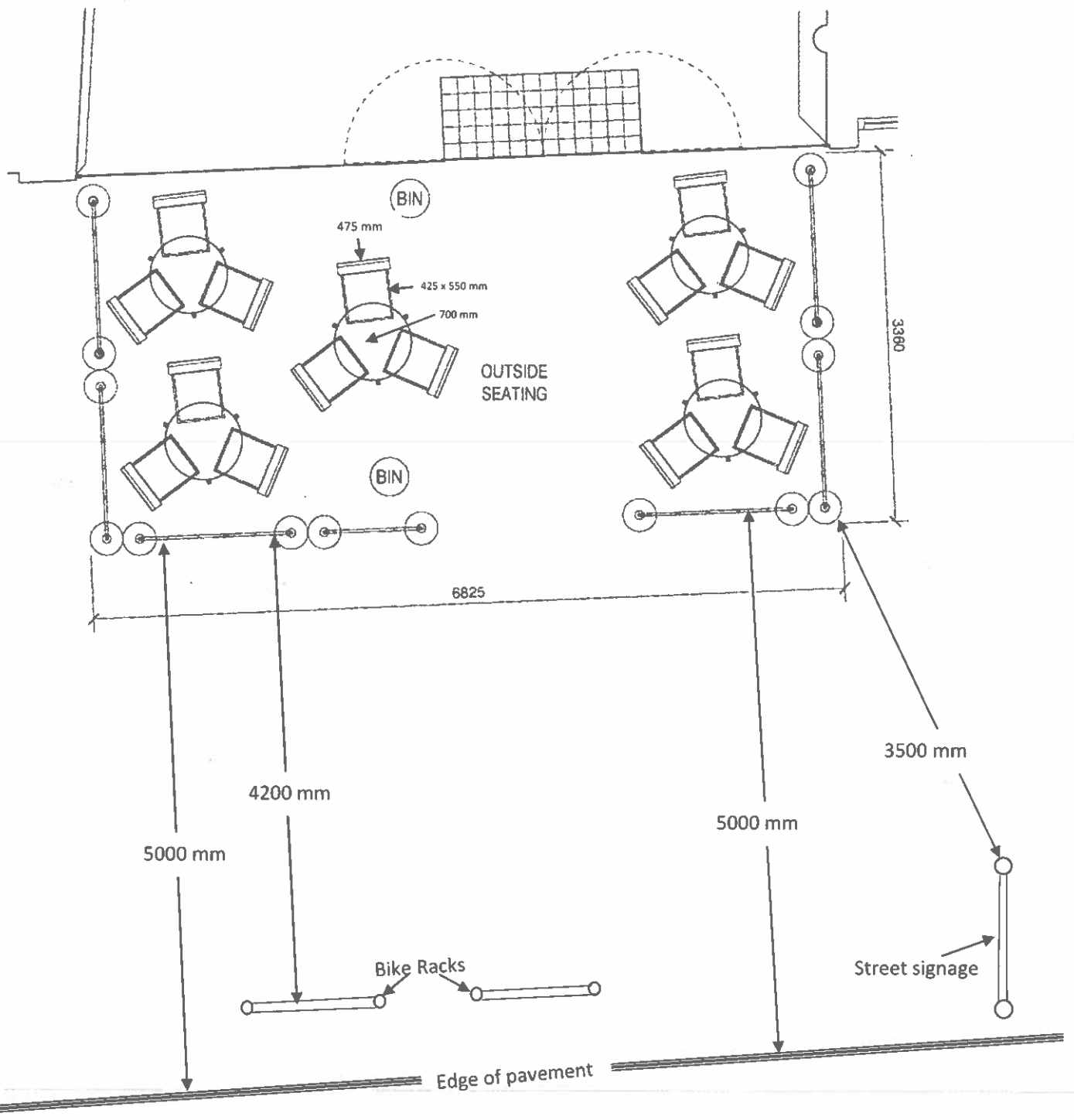
OUTSIDE SEATING LAYOUT FOR S2098: GREGGS, 92 TOTTENHAM COURT ROAD, LONDON, W1T 4TL SCALE 1:50 @A4
