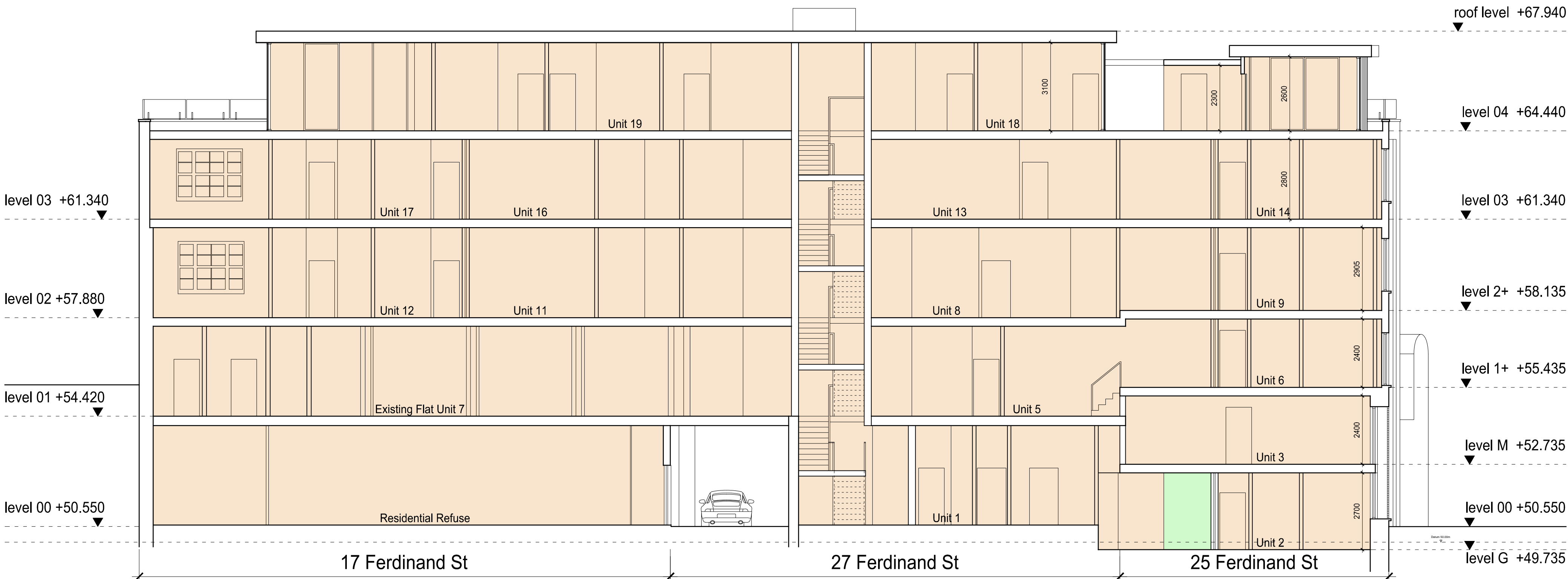
PROPOSED SECTION AA'
