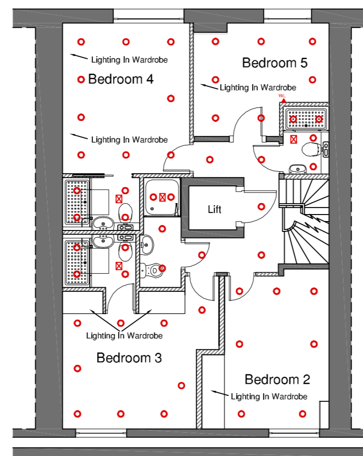
Proposed Third Floor
