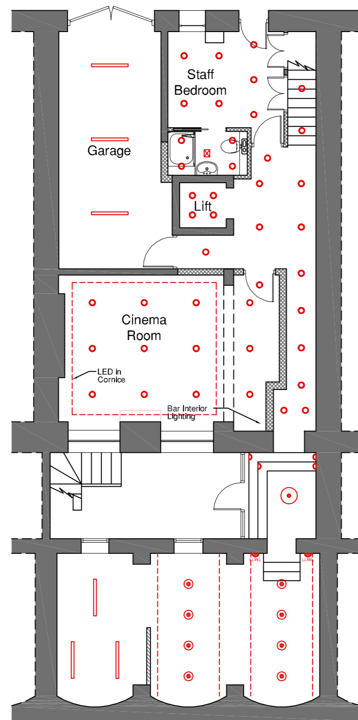
Proposed Lower Ground Floor
