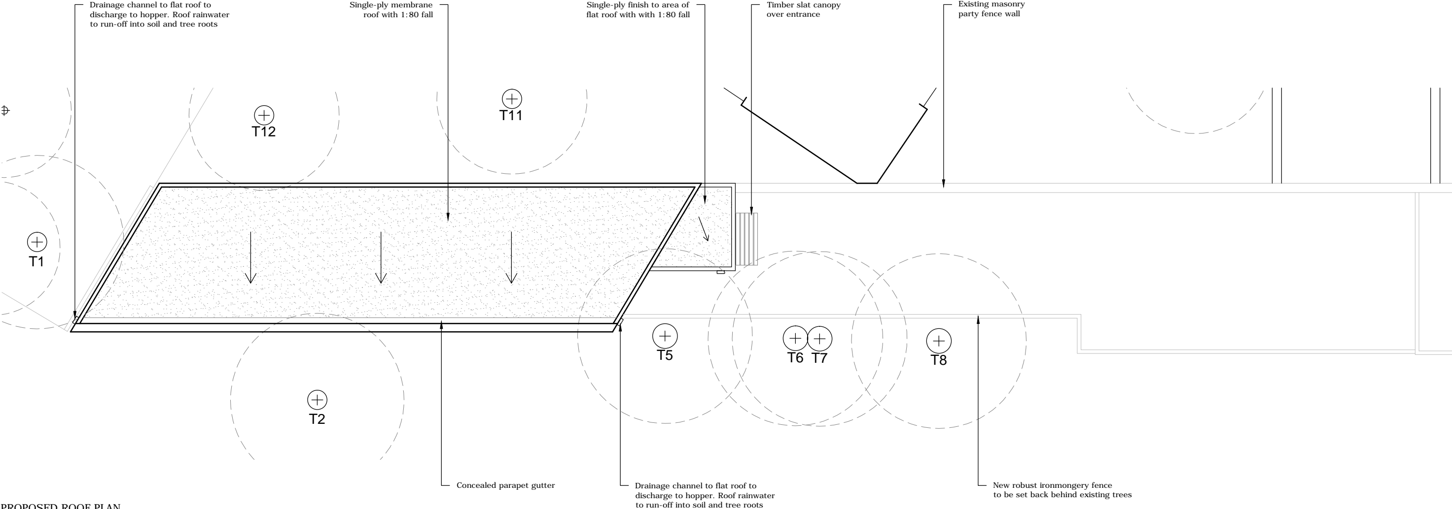
PROPOSED ROOF PLAN SCALE: 1:100
