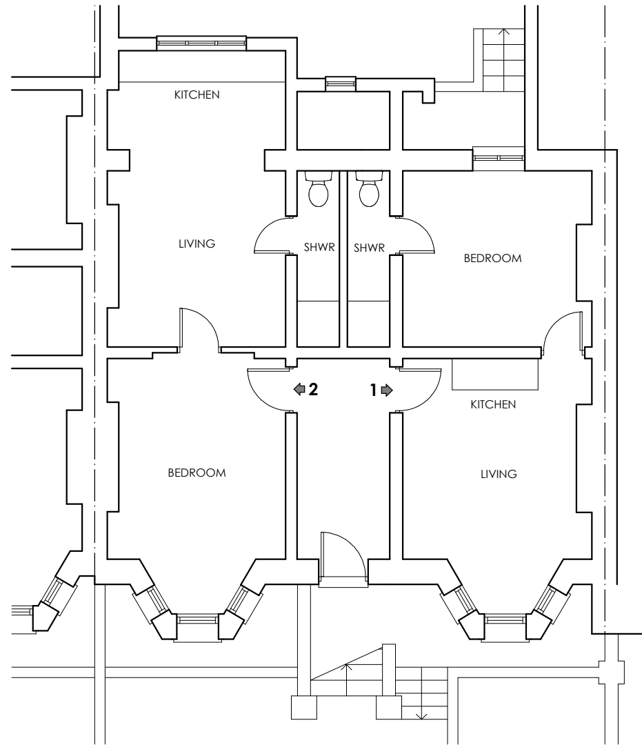
BASEMENT
