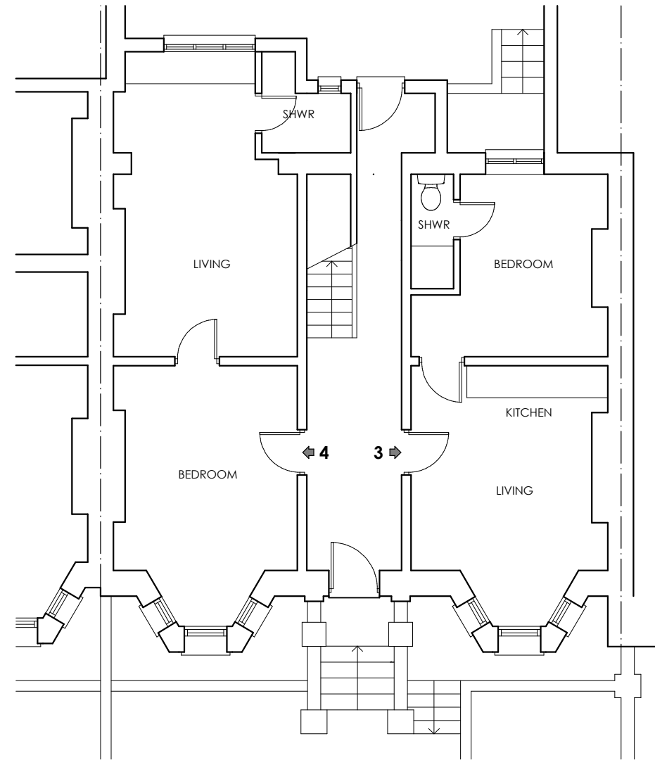
GROUND
