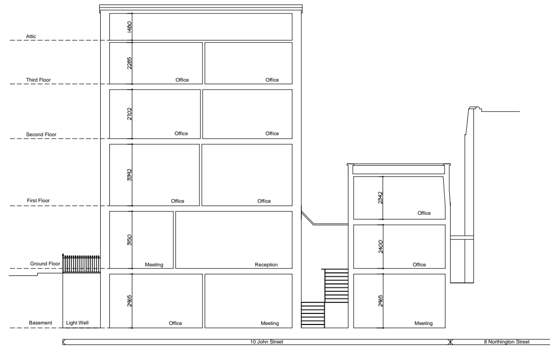
LONG SECTION
