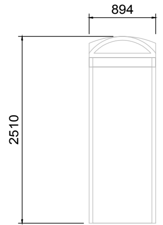
BACK ELEVATION Scale 1:50
