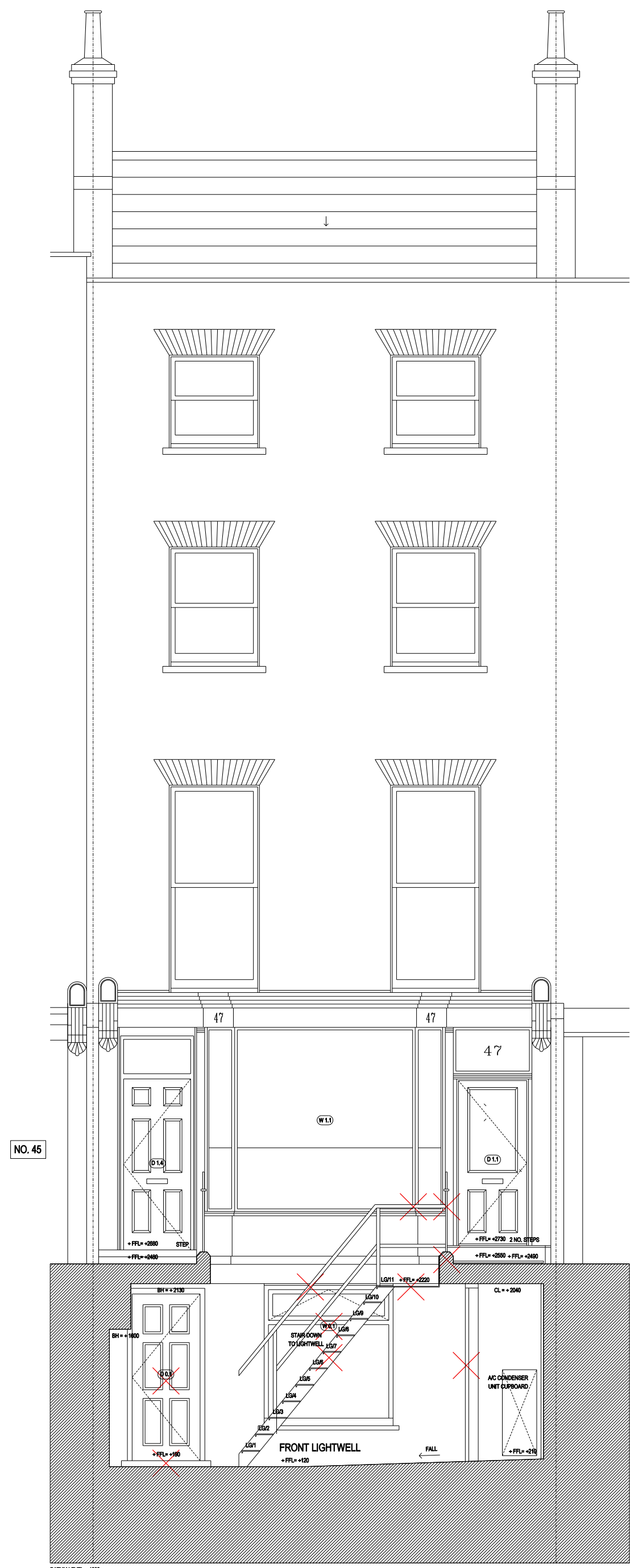
02 EXISTING SECTION 02 (15-01-02) Scale 1:50 (@A1 SIZE)
