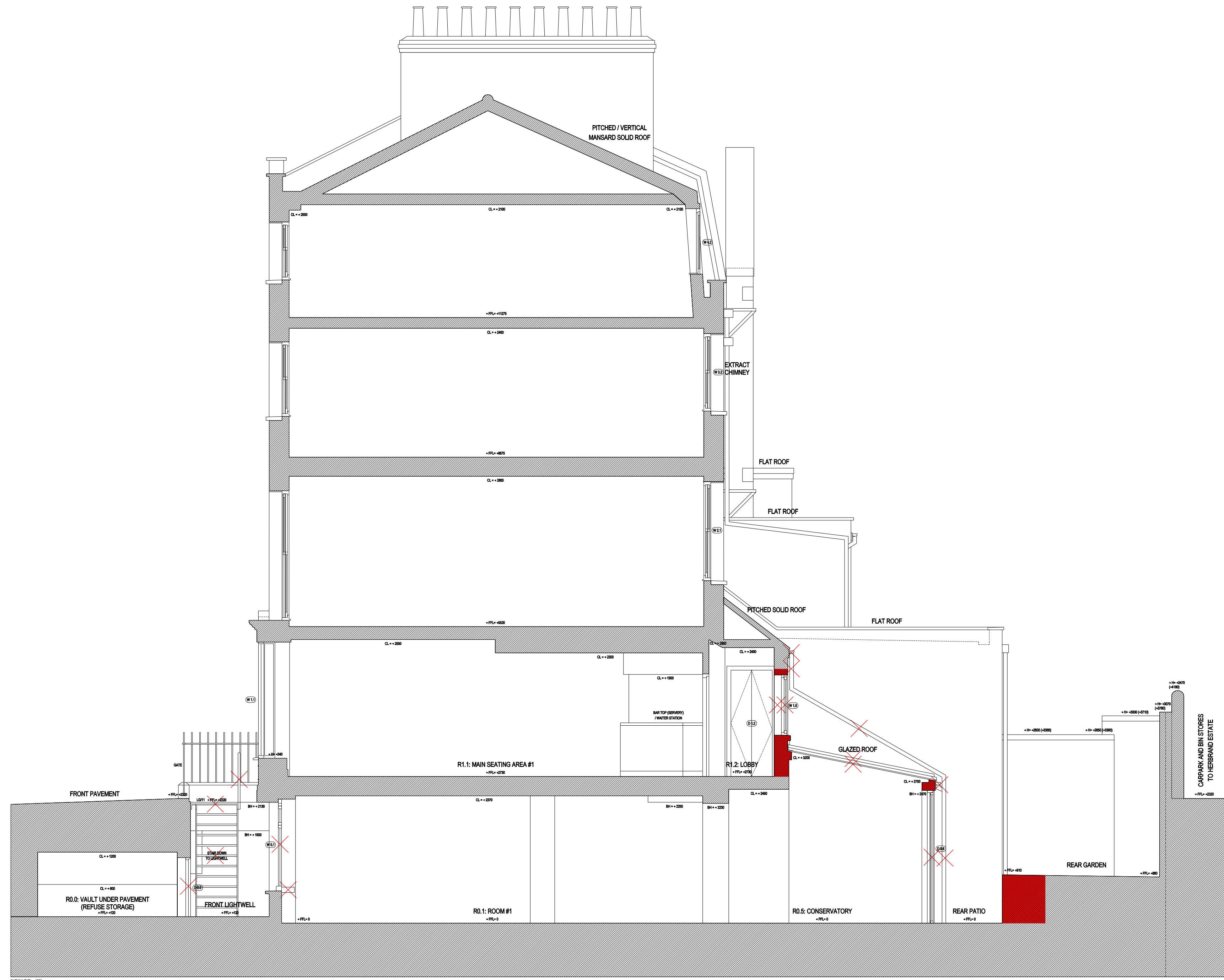
03 EXISTING SECTION 03 (15-01-02) Scale 1:50 (@A1 SIZE)
