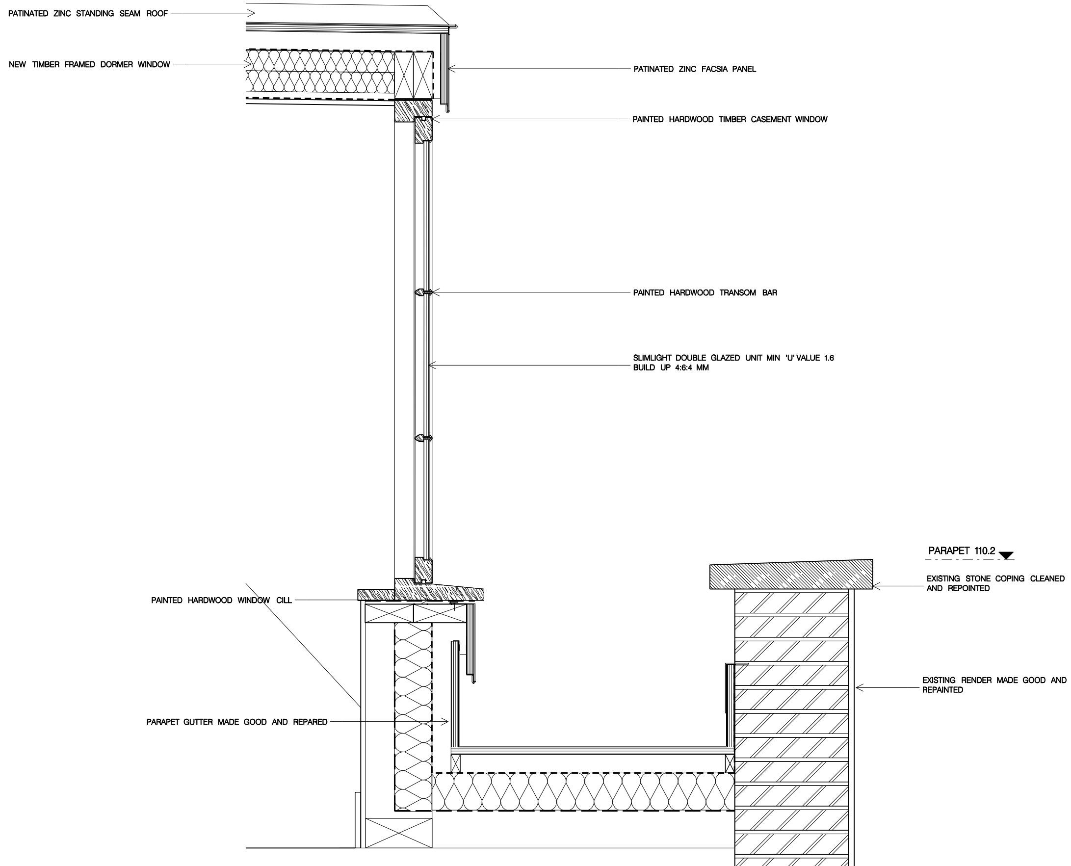
1 TYPICAL DORMER DETAIL TO EXISTING ROOF PL200
