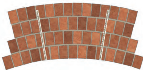
Stabilising bulging rubble-filled wall
