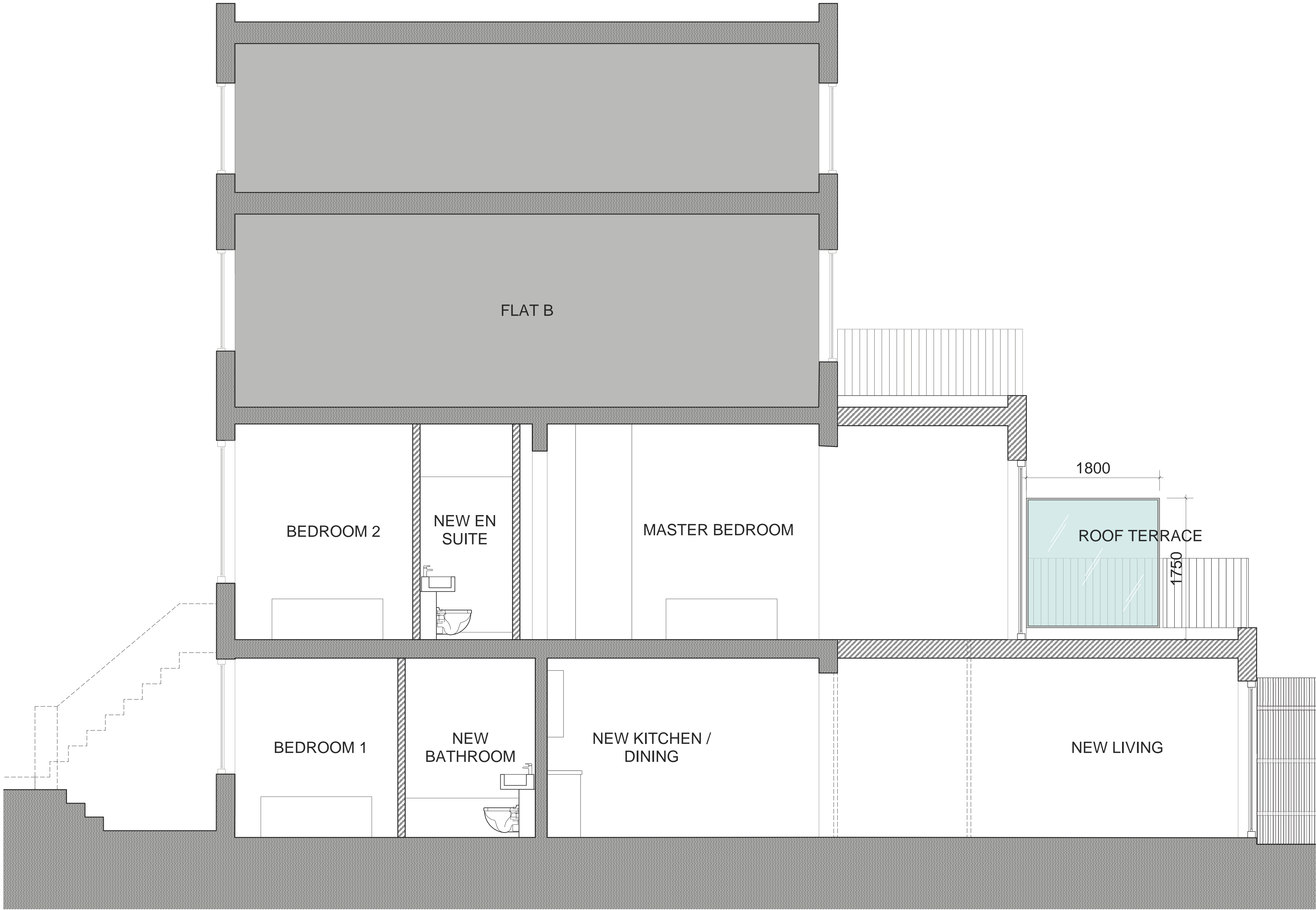
1 PROPOSED SECTION Scale: 1:25
