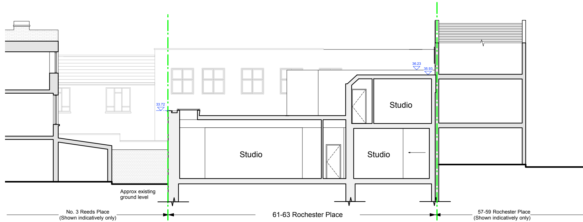
Existing Section E-E
