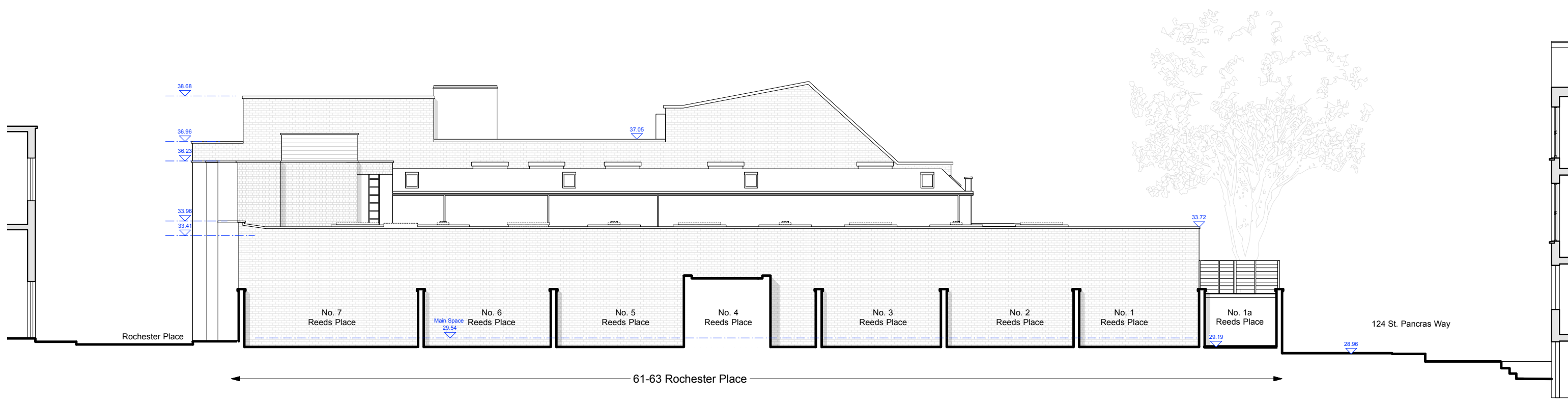
Side Elevation - North West
