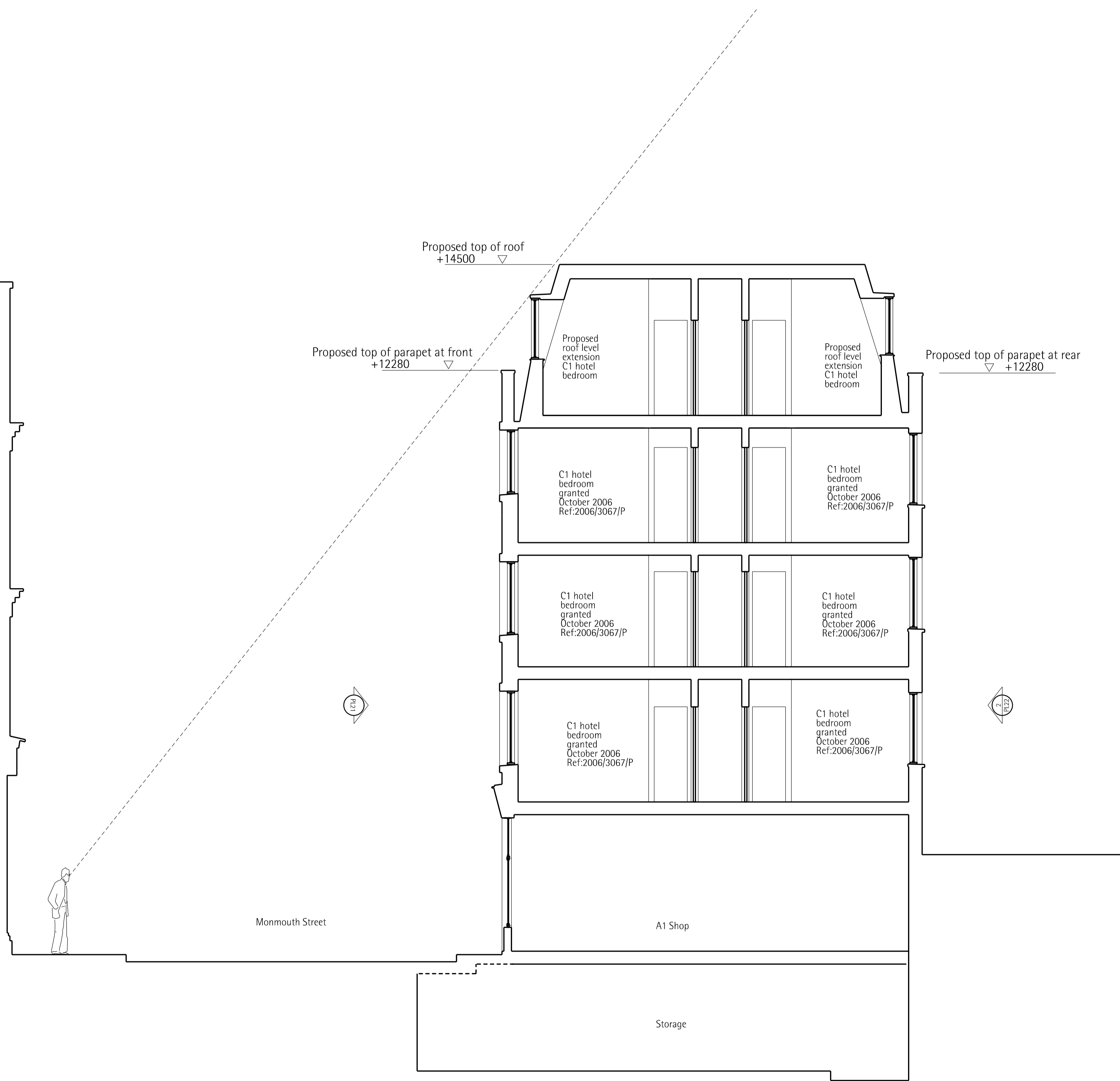
2. Proposed Section A Scale 1:50 @A1
