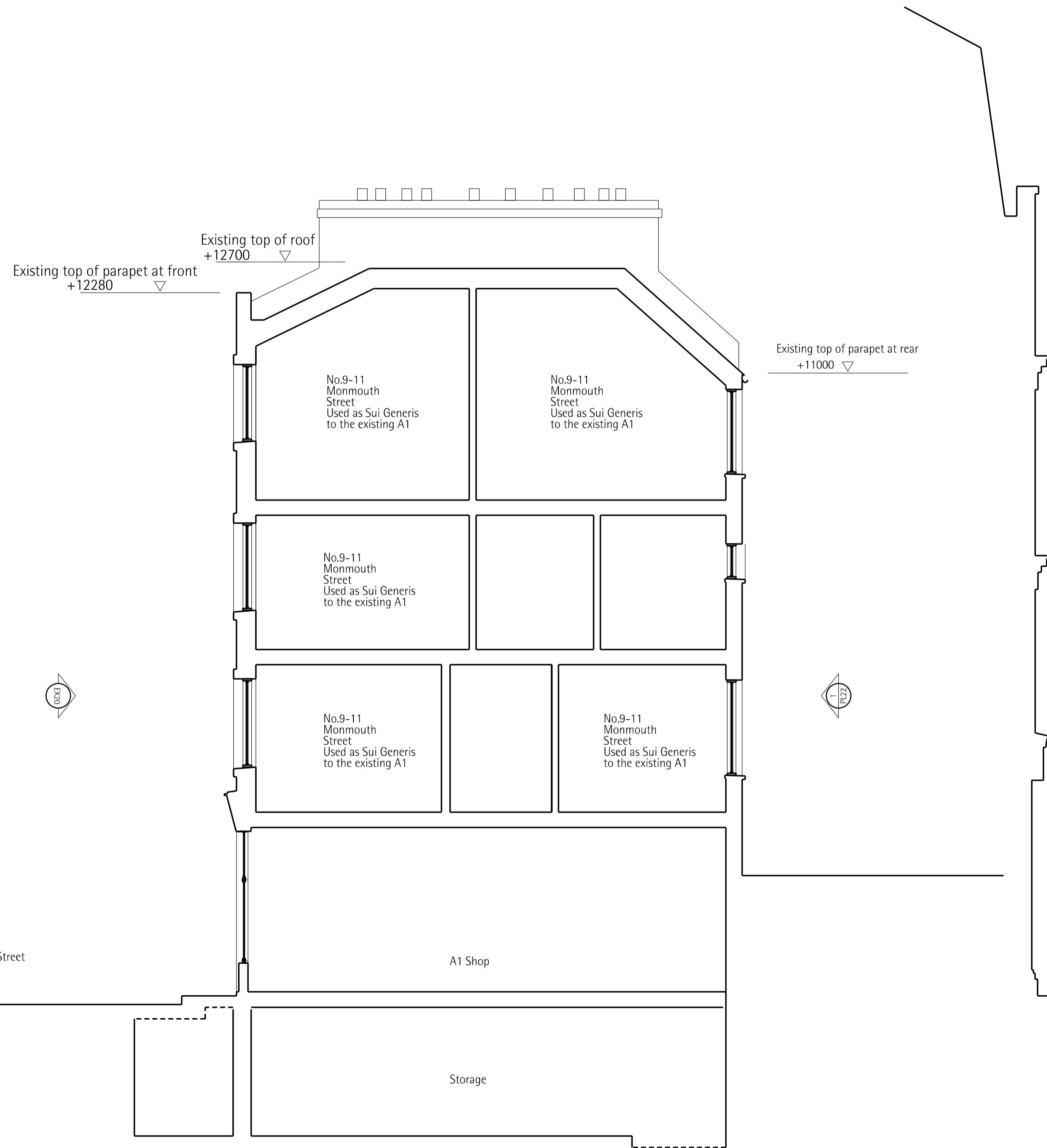
1. Existing Section A Scale 1:50 @A1
