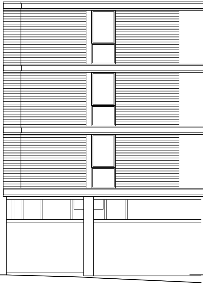
Existing (north elevation)
