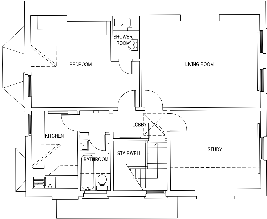
EXISTING SECOND FLOOR PLAN Scale 1:50@A1
