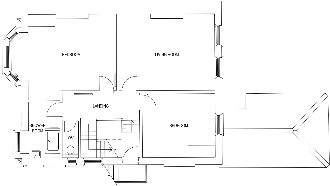
EXISTING FIRST FLOOR PLAN Scale 1:50@A1
