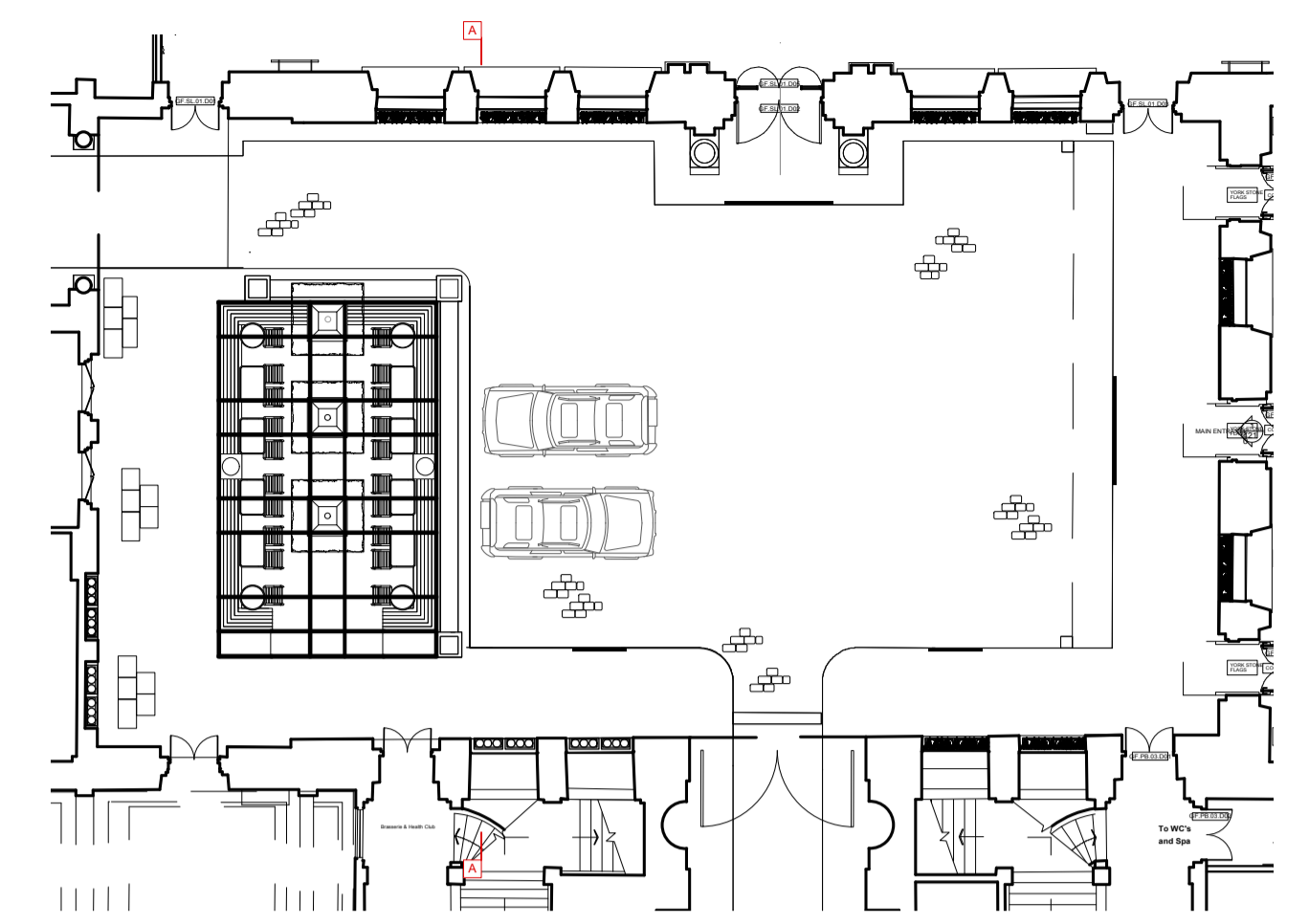
002 Key plan Rosewood Hotel 1:200 @ A1
